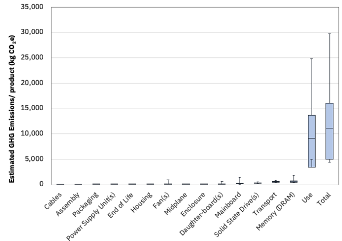
Figure 2: Uncertainty in the PCF estimate for the IBM® Storage FlashSystem 5200 typical product configuration listed in Table 1; the estimate has a total mean of 11,000 ± 7,000 kg CO 2 e over a use period of 5 years.
