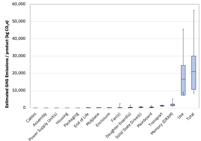
Figure 2: Uncertainty in the PCF estimate for the IBM® Storage FlashSystem 7300 typical product configuration listed in Table 1; the estimate has a total mean of 22,000 ± 12,000 kg CO 2 e over a use period of 5 years.
